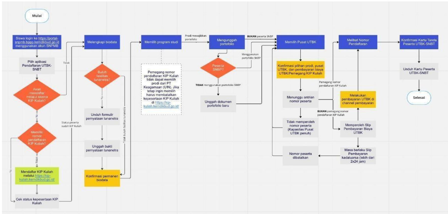
Figure 3. UTBK-SNBT registration
